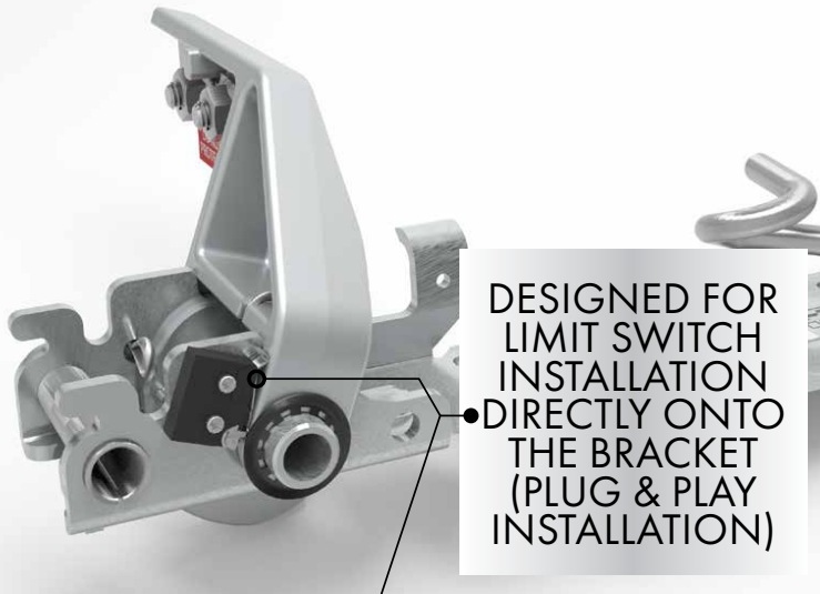
BURGLAR-RESISTANT DEVICE (# 181454)
